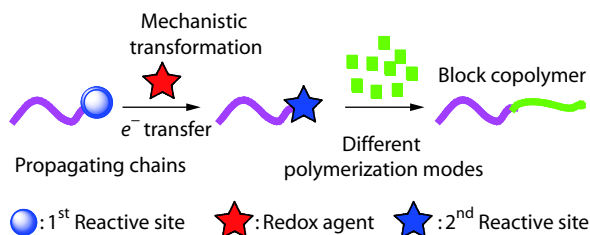
Scheme 1 Direct mechanistic transformation.
