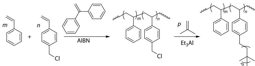
Scheme 3 Mechanistic transformation from iniferter to cationic polymerization.
